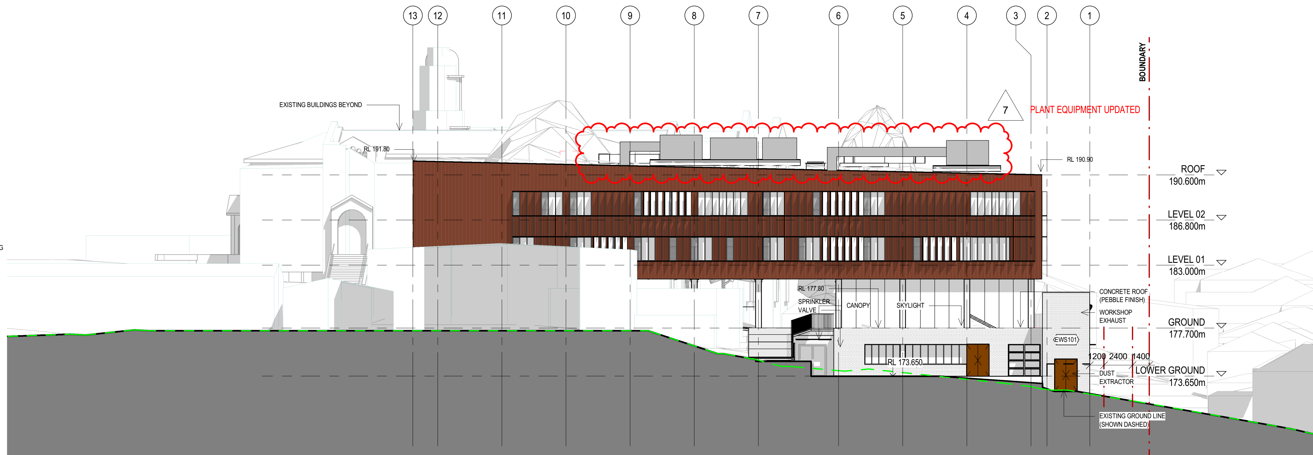
2 DA ELEVATION - EAST AR-T10_XX-01
